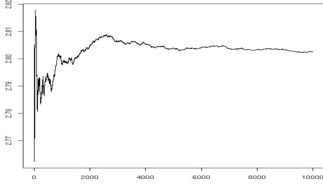
FIGURE 1. Convergence of the first coefficient of \hat{\theta} in an experiment with \sigma^2 = 1 , p = 8 . We represent the first coordinate of \frac{1}{N-b_0+1} \sum_{t=b_0}^N \hat{\theta}_{I(t)} as a function of N = b_0, \dots, T .
