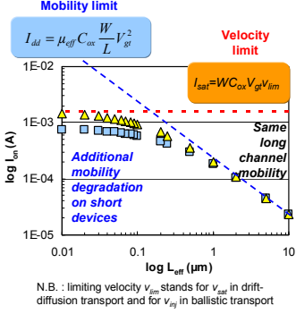
Fig. 2: Strong mobility degradation on short devices prevents from reaching the velocity limit, i.e. maximum on-current.
