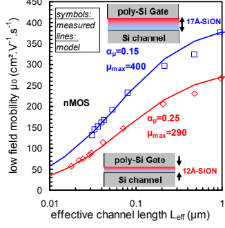
Fig. 7: Comparison of electron mobility between two SiON gate oxide thicknesses. Thinner 12Å oxide is more degraded than 17Å.
