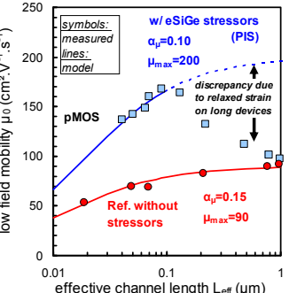
Fig. 11: Comparison of hole mobility between unstrained reference and locally strained device with eSiGe S/D stressors.
