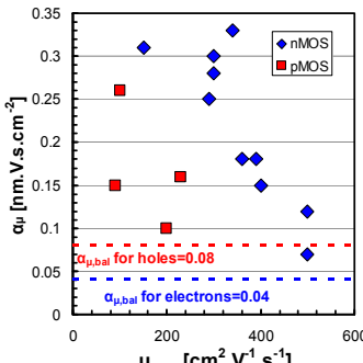
Fig. 14: \alpha_\mu as a function of \mu_{max} clearly showing no universal correlation between \alpha_\mu & \mu_{max} .
