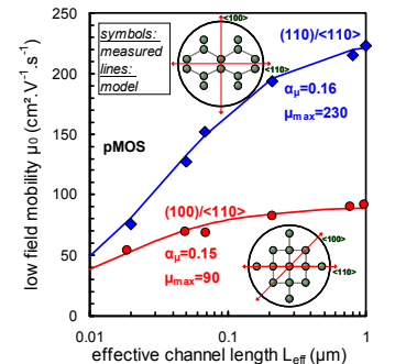
Fig. 12: Comparison of hole mobility between (100)/<110> device and (110)/<110> device with same poly/SiON gate stack.
