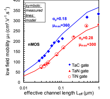
Fig. 8: Comparison of electron mobility between different metal gate materials. Nitrided metals are more degraded than not nitrided.
