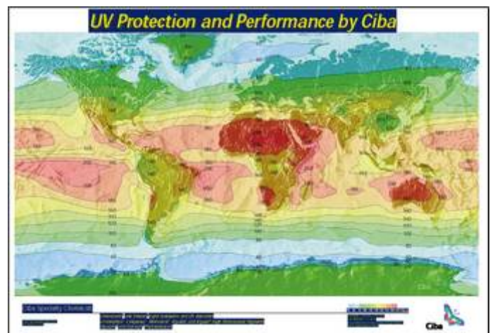
Figure 3. Example of information that is available for the whole world derived from the NASA Surface Radiation Budget project. This is the annual irradiance (energy flux). Units are \text{kLangley} . Values are to be multiplied by 1.33 to obtain \text{W}/\text{m}^2 . Copyright CIBA.
