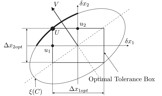
Figure 2: Tolerance Synthesis
