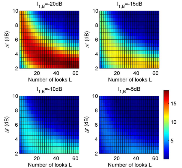
Fig. 8. Additional classification error due to ambiguity as a function of \Delta r and L for four values of I_{1,B} .
