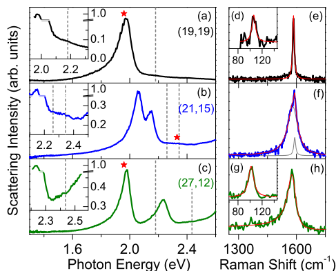
FIG. 3: (color online). (a-c) Rayleigh scattering spectra of individual suspended M -SWNTs ( \text{mod}(n-m), 3) = 0 ). The insets show details of the spectra near the expected positions of phonon side-bands (dotted lines). The stars in the Rayleigh spectra (a-c) indicate the laser energy for the Raman measurements. (d-h) Raman data. The RBM frequencies of (d) 106 \text{ cm}^{-1} and (g) 101 \text{ cm}^{-1} yield diameters of 2.60 nm and 2.75 nm, respectively 18 . (e, f, h) G mode spectra showing chirality dependent electron-phonon coupling, as expected for chiral metallic nanotubes 20 . Spectra in (d,e,g) are fit to Lorentzian profiles, while the fits in (f,h) are based on Fano profiles.
