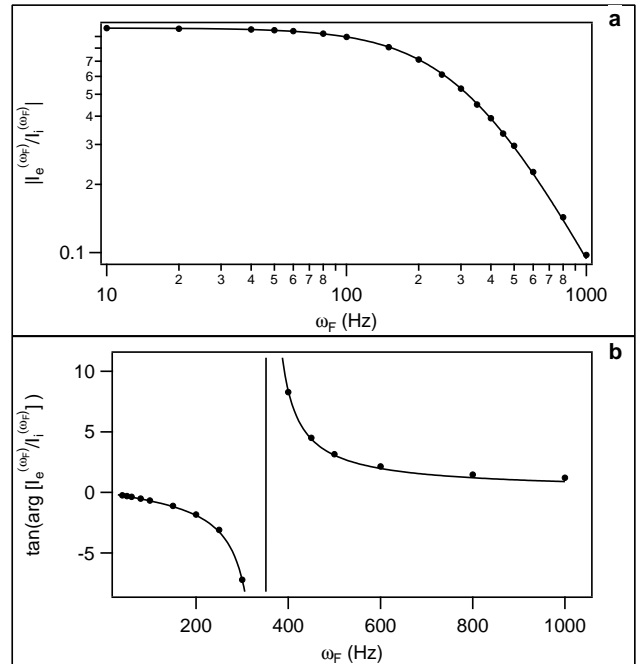
Fig. 5 Cavity response function towards the extraordinary beam. (a) Gain of the response function normalized to 1 at low frequency i.e. |I_e^{(\omega_F)} / I_i^{(\omega_F)}| as a function of the modulation frequency \omega_F . Data are fitted by the gain of a second-order low pass filter. (b) Tangent of the phase delay between I_e^{(\omega_F)} and I_i^{(\omega_F)} as a function of the modulation frequency. Data are fitted by the phase delay of a second-order low pass filter.
