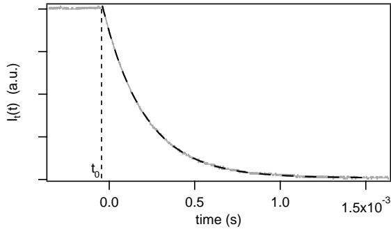
Fig. 2 Time evolution of the intensity of the ordinary beam (gray line). The laser is switched off at t = t_0 . Experimental data are fitted by an exponential decay (black dashed line) giving a photon lifetime of \tau = (245 \pm 10) \mu\text{s} and a finesse of F = (105 \pm 5) \times 10^3 .
