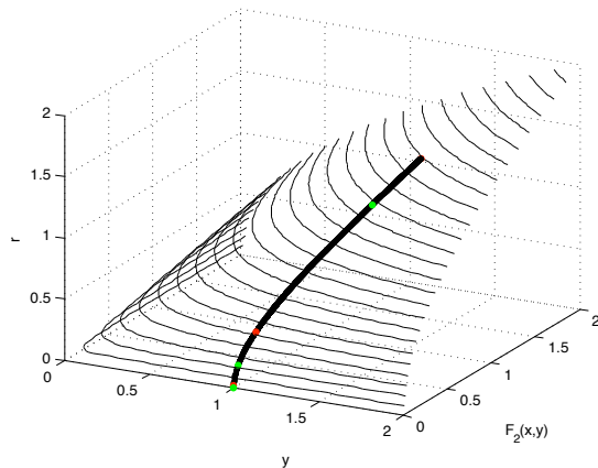
Figure 4.1: Evolution of (y, F_2(x, y), r) .
