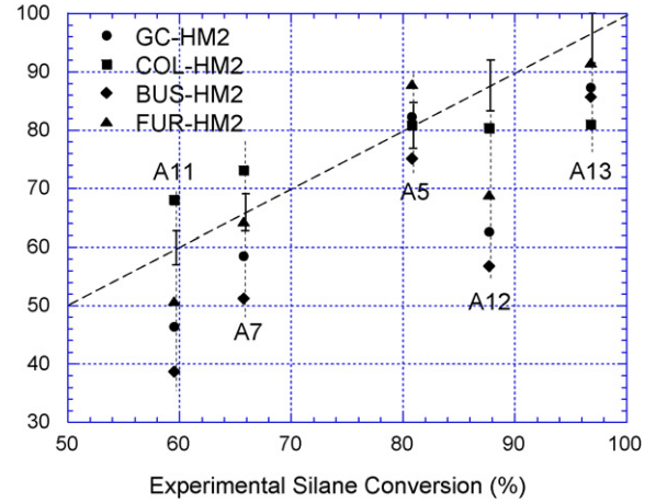
Fig. 7. Calculated silane conversions vs. experimental silane conversions.
