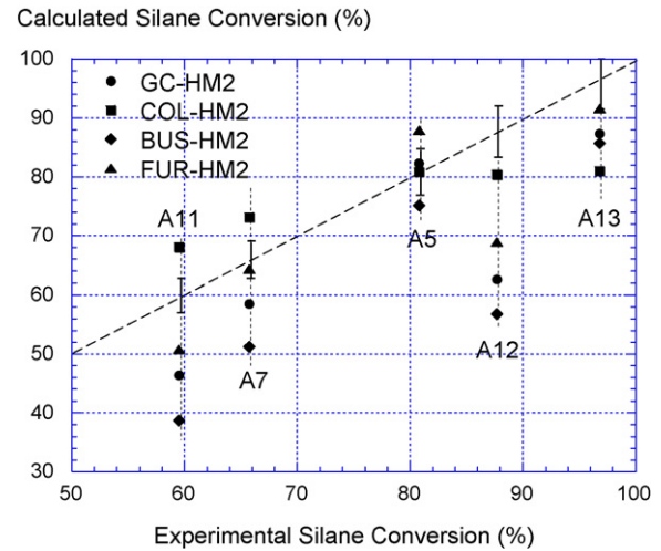
Fig. 7. Calculated silane conversions vs. experimental silane conversions.
