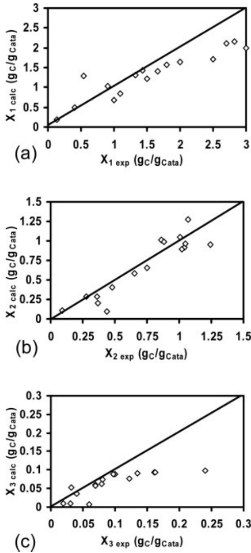
Figure 3. Comparison between experimental and simulated productivities (runs Cin1 to Cin25). (a) X_1 MWCNTs productivity, (b) X_2 ethane productivity, and (c) X_3 methane productivity.
