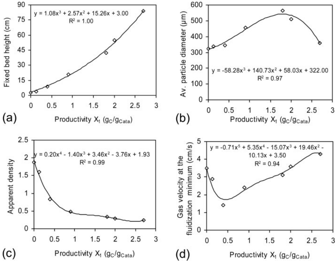
Figure 2. Physical laws of evolution of the fluidized bed and of the particles features with X_1 the MWCNTs productivity. (a) Fixed bed height, (b) average diameter of particles, (c) apparent density, and (d) minimum fluidization gas velocity.
