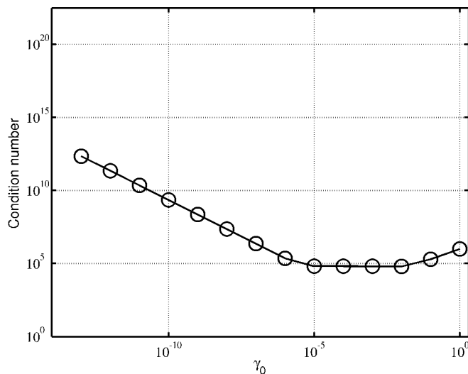
Figure 8: Sensitivity of the condition number of the Newton tangent linear system for different values of \gamma_0 for the P_1/P_2 experiment and h = 2mm .
