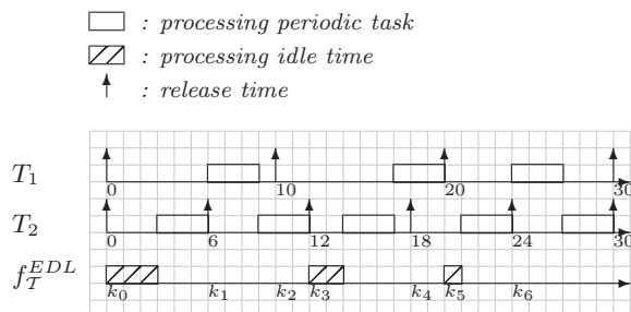
Figure 3: f_{\mathcal{T}}^{EDL} computation produced at time zero
