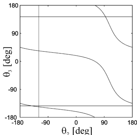
Figure 5: Joint Space of the Non-Generic 3R Manipulator defined by: d_2 = 1, d_3 = 2, d_4 = 2.5, r_2 = 1, r_3 = 0, \alpha_2 = -60^\circ, \alpha_3 = 90^\circ
