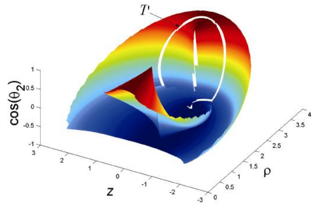
Figure 10: T lies in a Region of Feasible Paths
