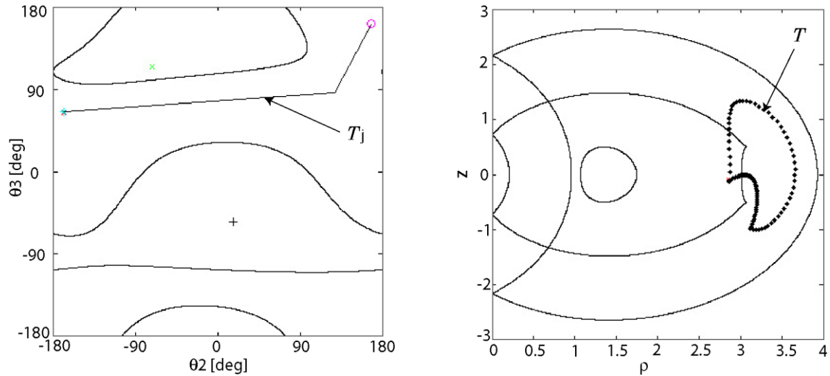
Figure 16: Manipulator d_2 = 1 , d_3 = 0.6 , d_4 = 2 , r_2 = 1 , r_3 = \mathbf{0.5} , \alpha_2 = -90^\circ , and \alpha_3 = 90^\circ : T is Path Feasible
