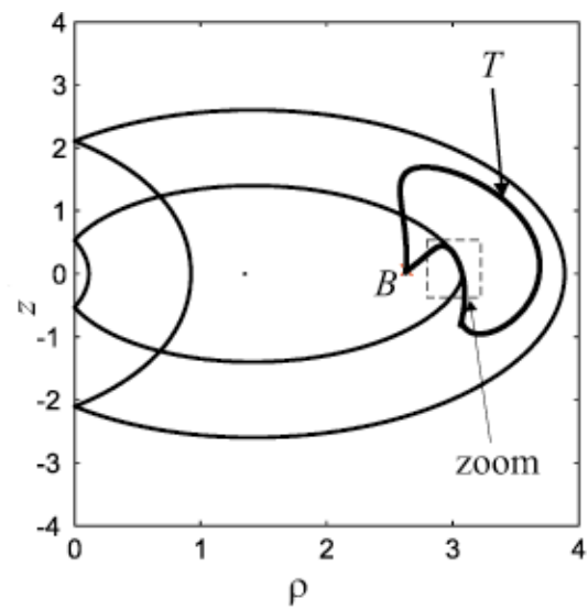
Figure 11: T is not Path Feasible
