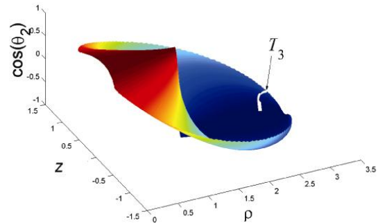
Figure 15: T_3 lies in a Region of Feasible Paths
