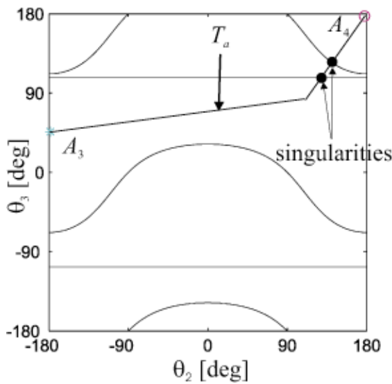
Figure 11: T is not Path Feasible
