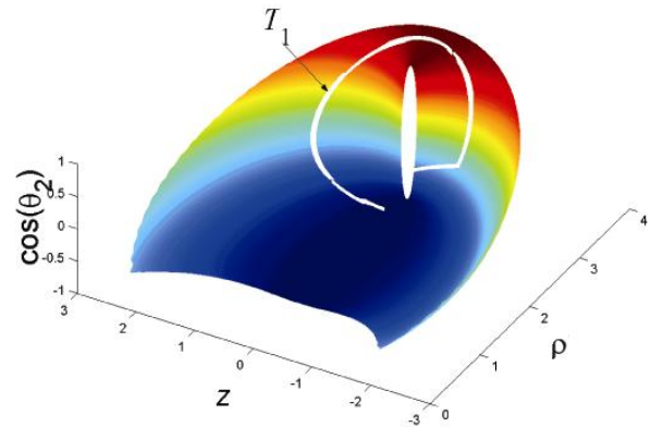
Figure 13: T_1 lies in a Region of Feasible Paths
