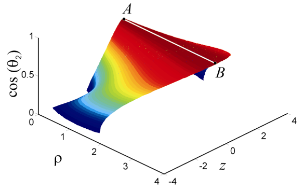
Figure 20: Image of aspect A_2 : Region 2 of Feasible Paths
