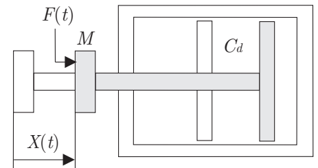
Figure 4. Damper
