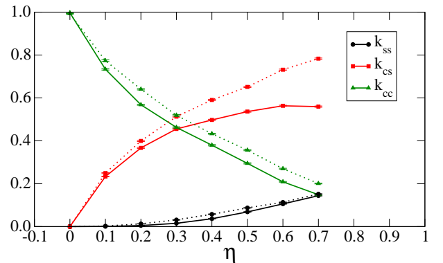
FIG. 29: Proportions of cap-to-cap ( k_{cc} ), cap-to-side ( k_{cs} ) and side-to-side ( k_{ss} ) contacts in the strong (plain line) and weak (dashed line) networks as a function of \eta in the residual state. The error bars represent the standard deviation in the residual state.
