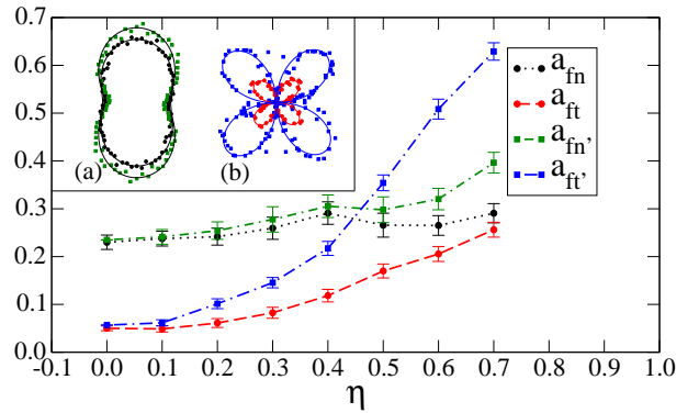
FIG. 17: Normal and tangential force anisotropies a_{fn} and a_{ft} and radial and orthoradial force anisotropies a_{fn'} and a_{ft'} as a function of \eta in the residual state. The error bars represent the standard deviation in the residual state. The inset shows the angular average functions \langle f_n \rangle(\theta) and \langle f_{n'} \rangle(\theta) in black and green, respectively, (a) and \langle f_t \rangle(\theta) and \langle f_{t'} \rangle(\theta) in red and blue, respectively, (b) for \eta = 0.7 calculated from the simulation data (points) together with the harmonic approximation (lines). The error bars represent the standard deviation in the residual state.
