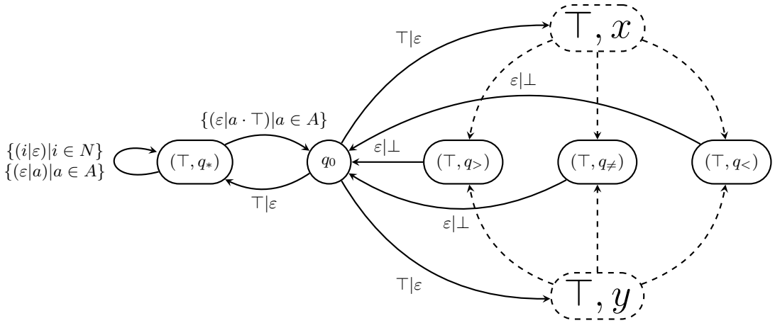
(b) Structure of the \top part of \mathcal{M}_{\mathcal{I}}
