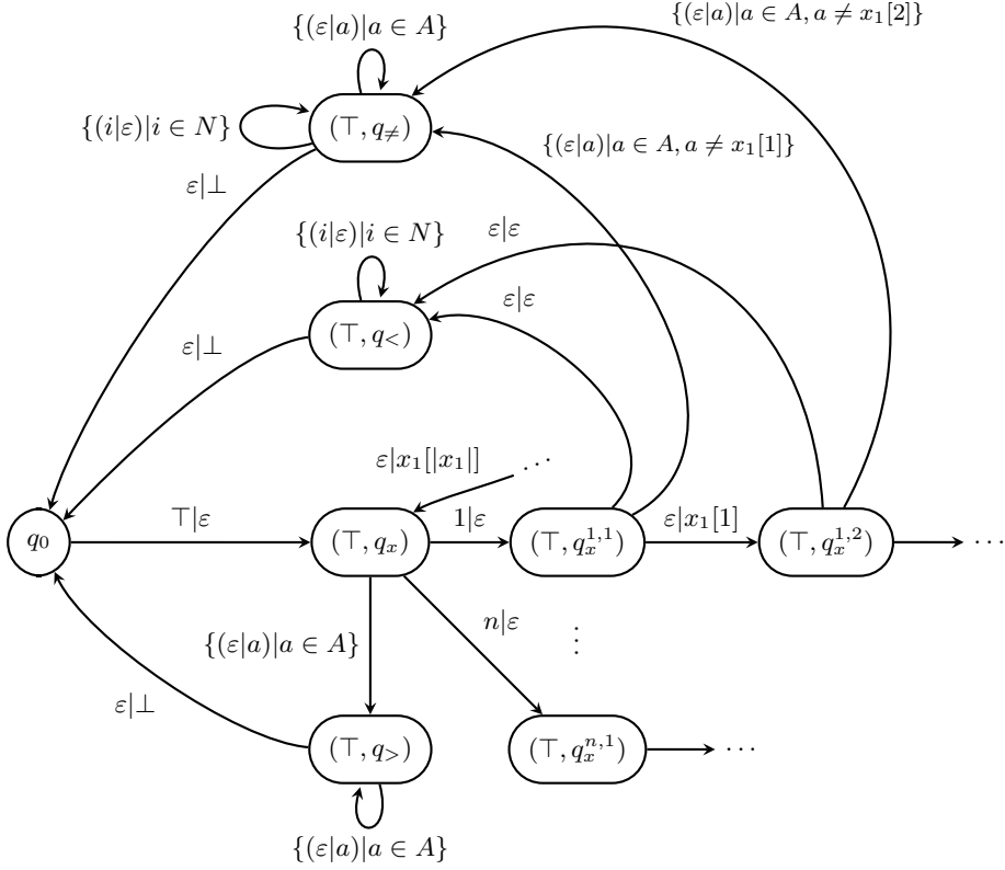
Fig. 9. Structure of the (\top, x) part of \mathcal{M}_{\mathcal{I}} that accepts \{(\top \cdot \sigma, u \cdot \perp) \mid u \neq x(\sigma)\}^* .
