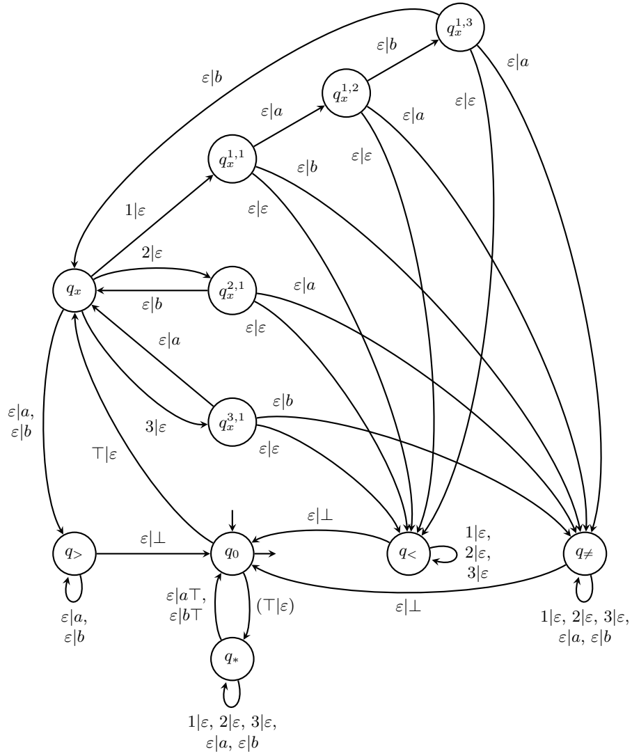
Fig. 11. Part of transducer \mathcal{M}_{\mathcal{I}_0} encoding PCP instance \mathcal{I}_0 . Only the \top - x quarter has been represented due to lack of space.
