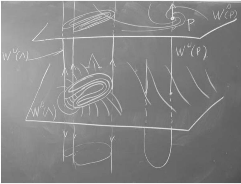
Figure 3: A robustly non-hyperbolic diffeomorphism with a robust cycle
