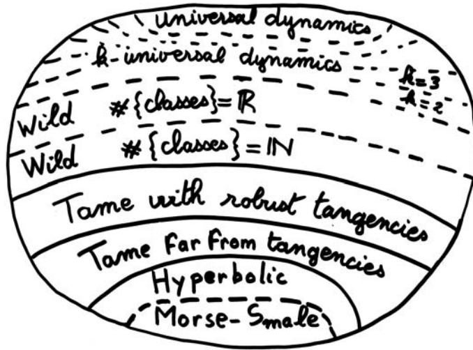
Figure 1: Conjectural map of Diff^1(M)
