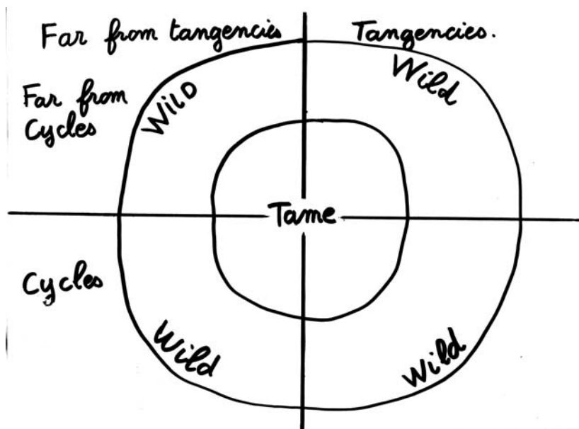
Figure 4: Splitting \text{Diff}^1(M) in 8 open regions
