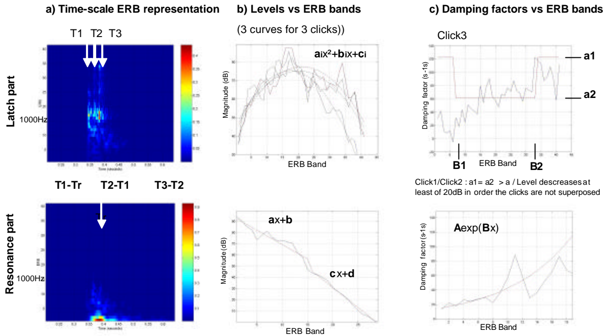
Figure 1.- Analysis - signal parameters (in bold). The upper part of the figure corresponds to the latch part of the signal, while the lower part corresponds to the resonant part of the signal. (a) Time-scale ERB decomposition (recombination of EMD modes). Detection of main impacts. (b) Levels vs ERB bands measured and approximated (dashed curves) for the 3 clicks of the latch part and for the impact of the resonance part. (c) Damping factors vs ERB bands measured and approximated (dashed curves).
