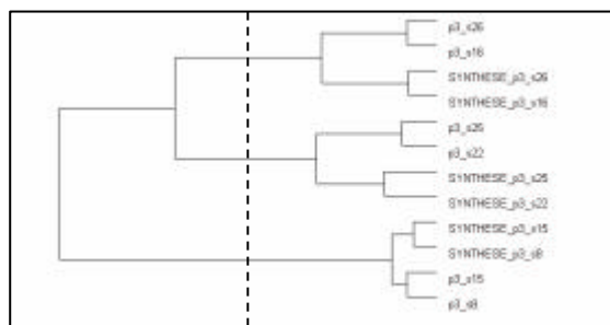
Figure 3.- Hierarchical Ascendant Classification of similarity ratings
