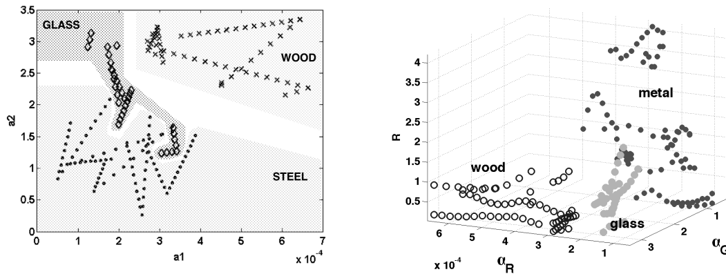
Figure 1: (a) Calibration of the damping parameters \alpha_G and \alpha_R , from the typical sounds represented for each material: Wood ( \times ), Glass ( \diamond ) and Metal ( \bullet ). Hence, a specific domain was determined for each material category. (b) Position of typical sounds (empty circles for Wood, grey circles for Glass and black circles for Metal) in a 3D space defined by the 2 damping parameters \{\alpha_G, \alpha_R\} and the roughness R .
