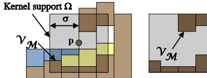
Figure 5: Evaluation of the convolution function: i(\mathbf{p}) is defined as the volume of material \mathcal{V}_{\mathcal{M}} inside the compact support \Omega of the kernel function.
