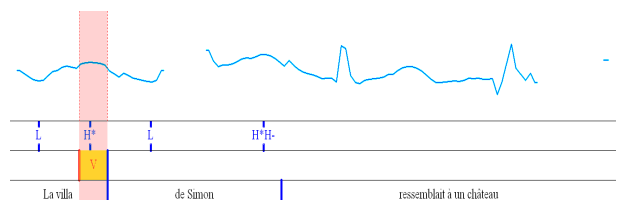
Figure 6 : F0 curve for the utterance La villa de Simon ressemblait à un château . ‘Simon’s house looked like a castle’ produced by one of our speakers at fast speech rate.
