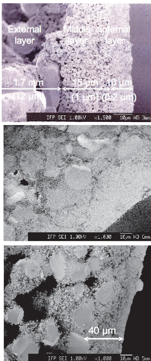
Figure 2 Cross-section SEM images of (from top to bottom): tubular tri-layered support S-0.2 (0.2 μm top-layer pore size), membrane M4 and membrane M7, both membranes formed on a S-0.2 support.
