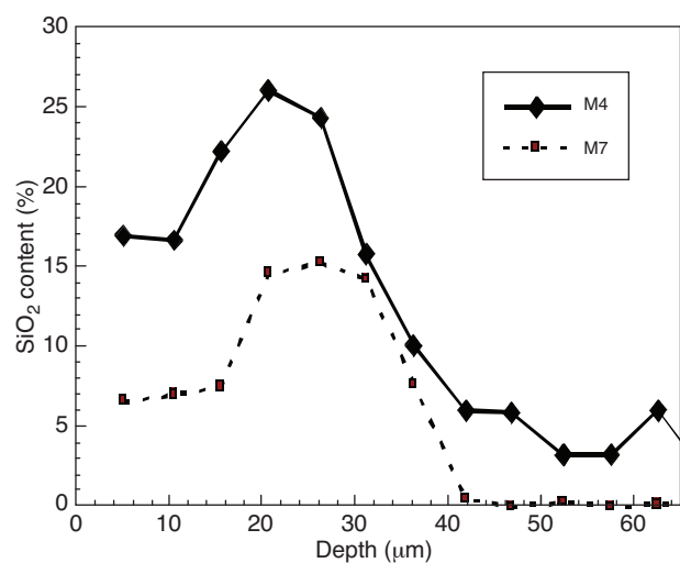
Figure 3 EPMA profiles of membranes M4 and M7.
