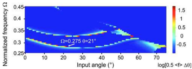
FIG. 2. (Color online) Design metric for slow light and ultrarefraction with r/a=0.2 and GK lattice termination.
