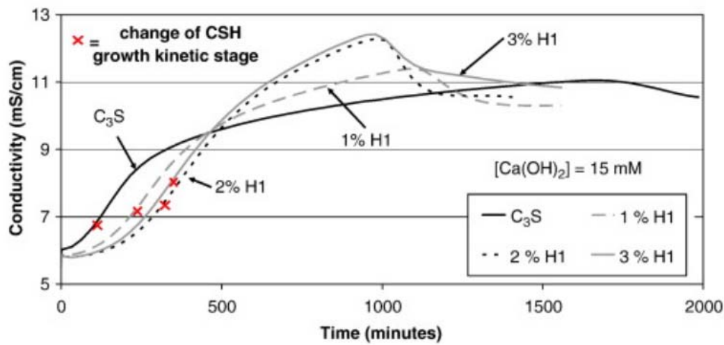
Figure 19: Conductometric curves of C_3S hydration admixed with various amount of H1 ( L/S = 100 , [Ca(OH)_2] = 20 \text{ mM} ).
