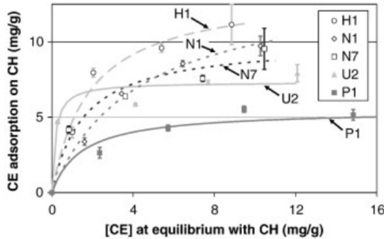
Figure 4: CE adsorption isotherms on CH after a 2 hour-exposure time ( L/S = 20 ).
