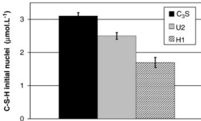
Figure 16: Impact of CE on the amount of initial nuclei of C-S-H precipitated after 30 min of C_3S hydration ( L/S = 100 , P/S = 2\% , [Ca(OH)_2] = 20 mM, volume of 100 mL).
