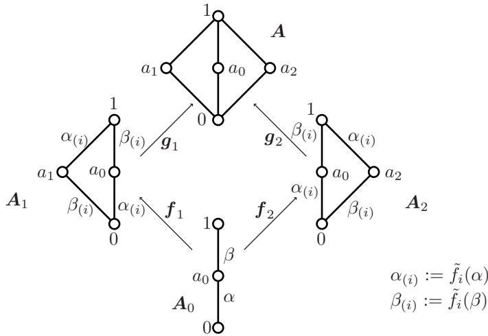
Fig. 5.2 A square in Metr unliftable with respect to \Psi and \mathbf{Metr}^\Rightarrow
