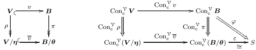
Fig. 4.2 Proving that \varphi \circ \text{Con}_c^{\mathcal{V}} v is ideal-induced
