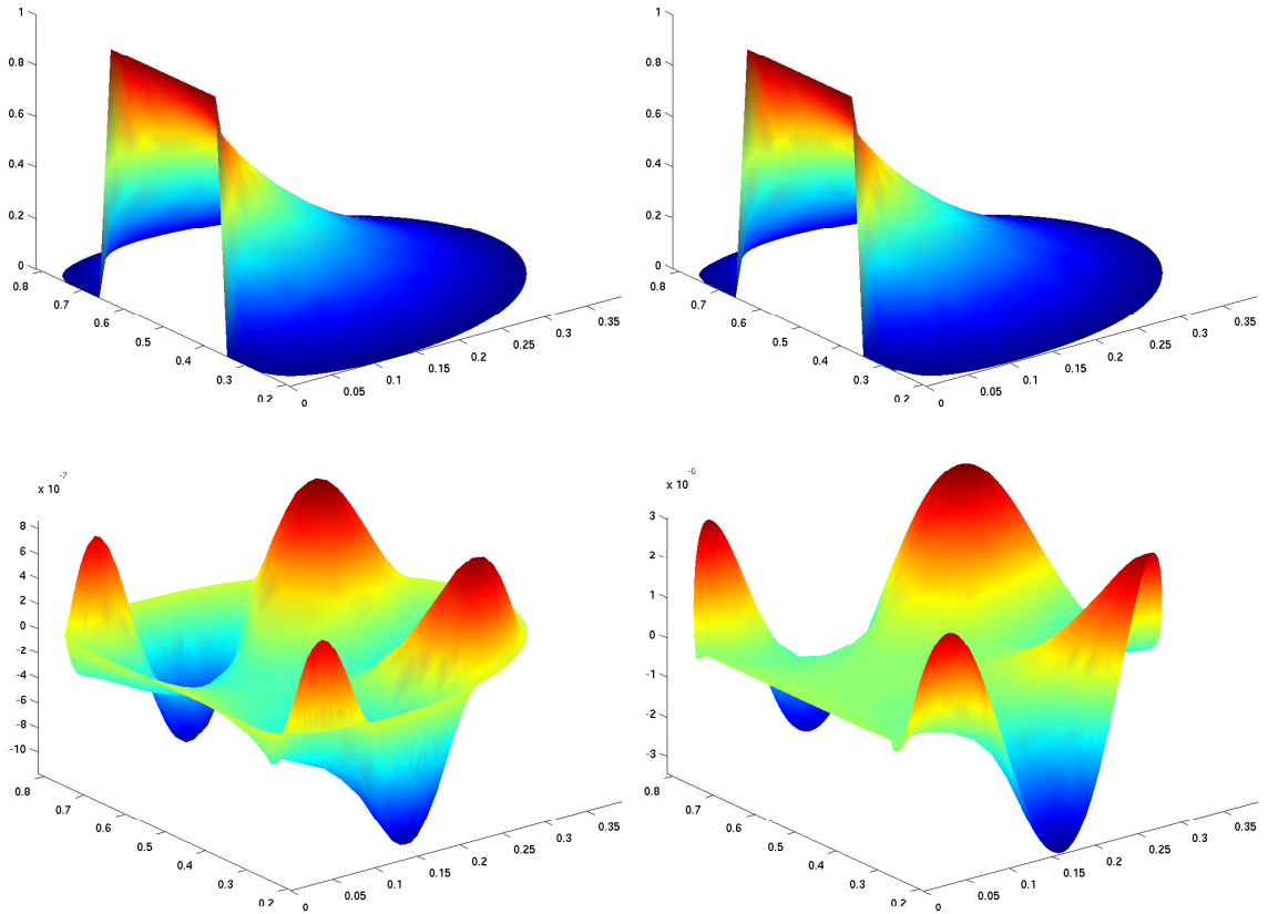
Figure 5: Solutions u_1 (top left), u_{2,\varepsilon} (top right), p_1 (bottom left), p_2 (bottom right) in the optimal domain.
