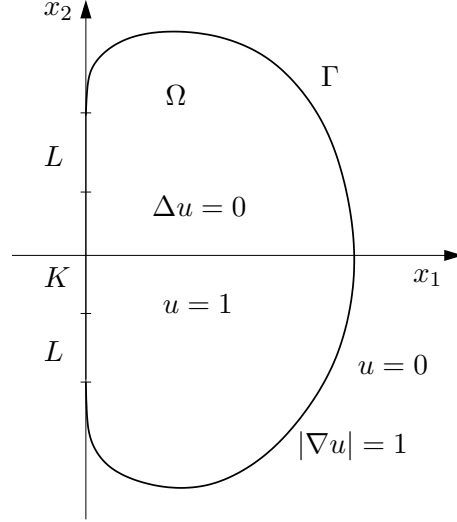
Figure 1: The domain \Omega in dimension two.
