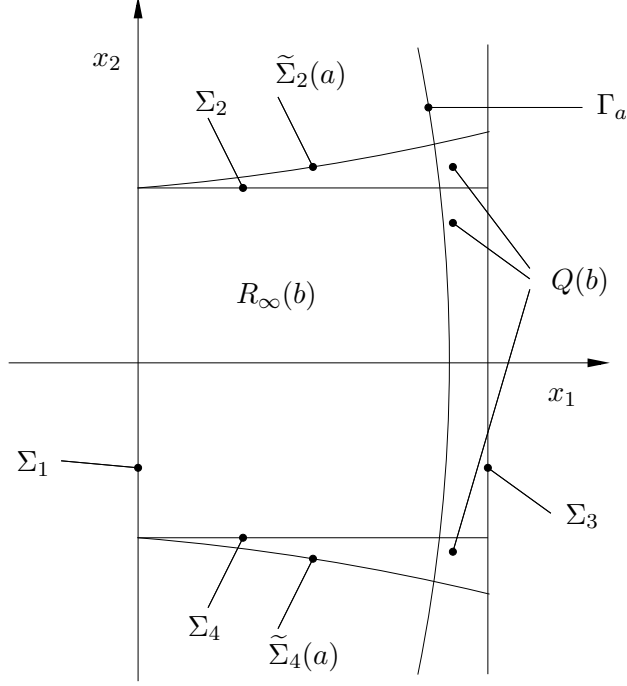
Figure 2: The sets R_\infty(b) and Q(b) .
