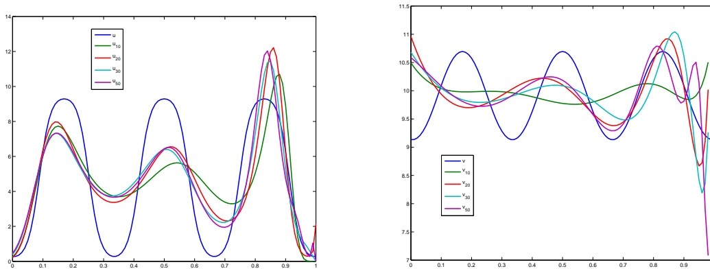
Figure 2: Smooth approx. for u (left) and v (right) for M \in \{10, 20, 30, 50\} for nonlinear ODE (12)
