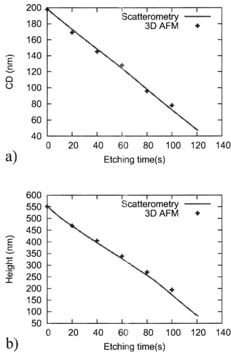
FIG. 6. Real time measurement results (solid line): (a) CD and (b) height of resist feature vs the processing time in HBr/O 2 with bias power. 3D AFM data (cross shape markers) are shown for reference.
