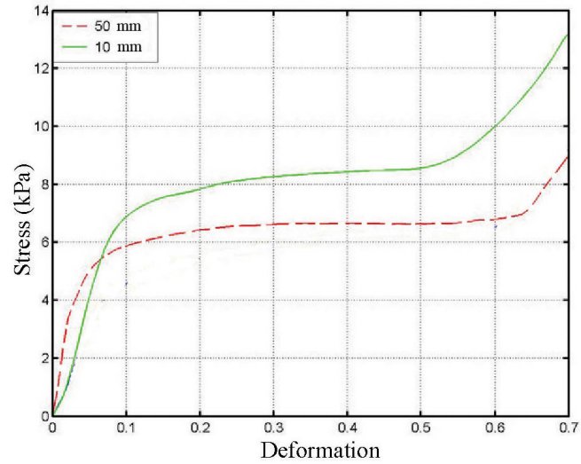
FIGURE 3. Comparison of the average force-elongation curves relative to five tests on 10 and 50 mm samples in confined compression.
