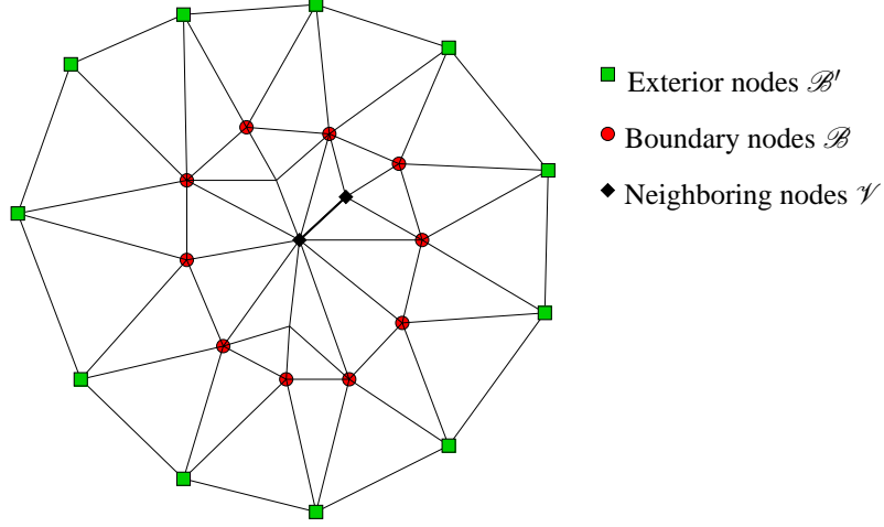
FIGURE 2. Boundary and exterior nodes in mesh \mathcal{T}
