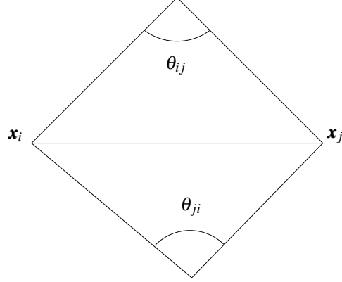
FIGURE 3. Angles and gradient norm in P_1(\mathcal{T})
