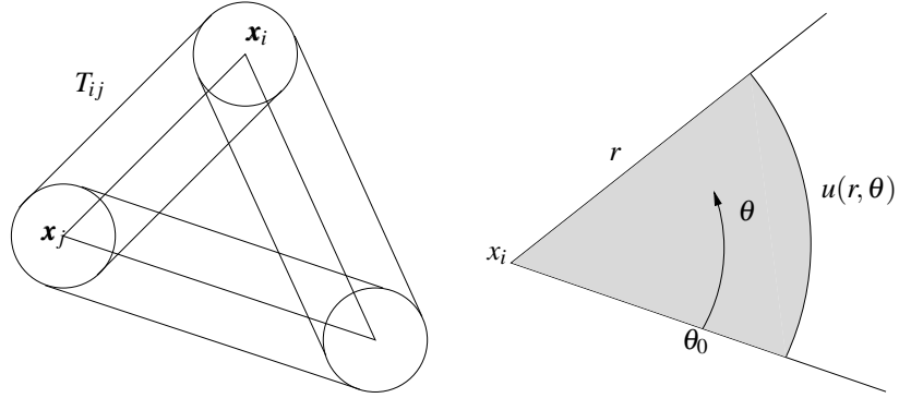
FIGURE 4. Tubes and their overlaps on the left, and estimate of the mean on a ball centered on an exterior edge on the right
