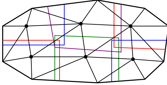
FIGURE 1. Domain decomposition with a coarse mesh
