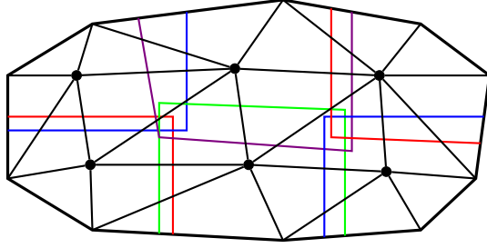
FIGURE 3.1. Domain decomposition with a coarse mesh
