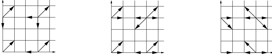
Figure 1: Three famous examples, known as Kreweras', Gessel's and Gouyou-Beauchamps' walks. They have been, and are still, the object of many studies, see, e.g. , [5, 12, 13], [4, 16, 17] and [8, 23], respectively.
