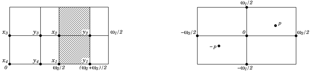
Figure 5: Domains of definition of \widehat{w} (on the left) and \overline{w} (on the right)
