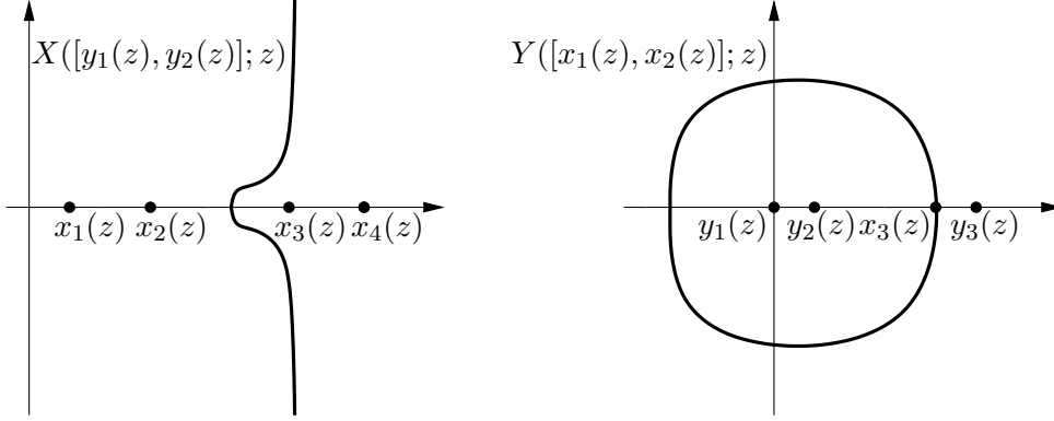
Figure 3: The curves X([y_1(z), y_2(z)]; z) and Y([x_1(z), x_2(z)]; z) for Gessel's walk
