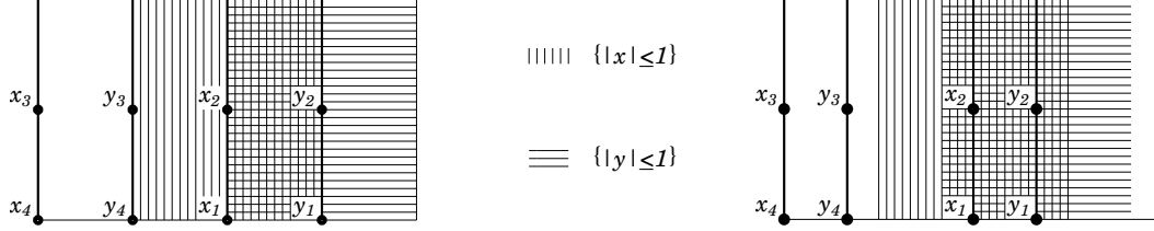
Figure 4: Examples of the parallelogram [0, \omega_2[ \times [0, \omega_1/\iota[ with its important cycles, on the left for \{N, E, S, W\} and on the right for \{N, E, SE, S, W, NW\}
