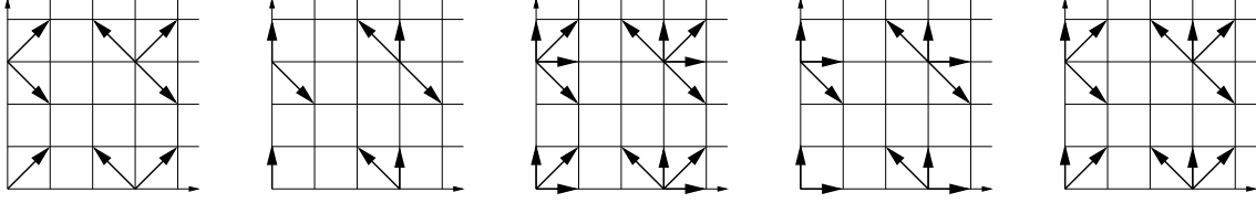
Figure 2: The 5 singular walks in the classification of [6]
