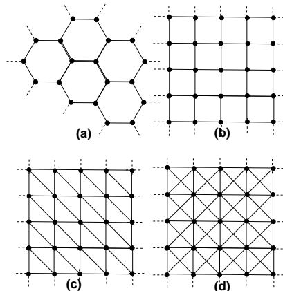
Figure 1 Grids studied in this paper: (a) G_3 , (b) G_4 , (c) G_6 and (d) G_8
