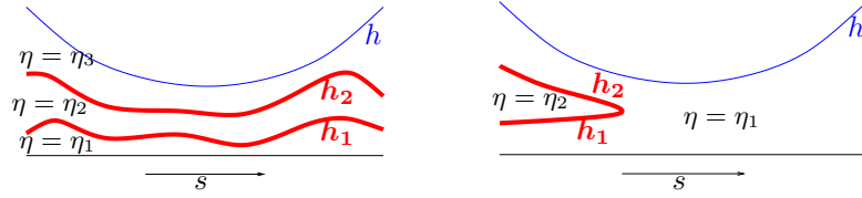
FIGURE 16. Three layers: (a) usual superposed fluids and (b) possible finger
