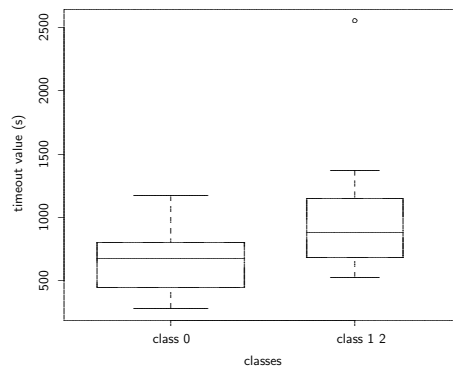
Figure 7: k -means classification into 3 classes after grouping classes 1 and 2.
