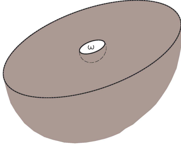
Figure 5: The domain \omega
