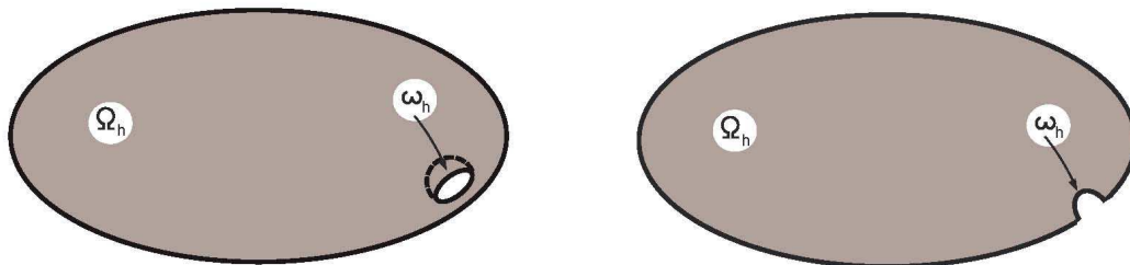
Figure 1: The domains \Omega(h) and \omega(h)
