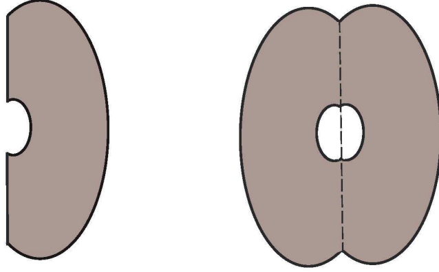
Figure 3: Mirror reflection of a domain with flat boundary
