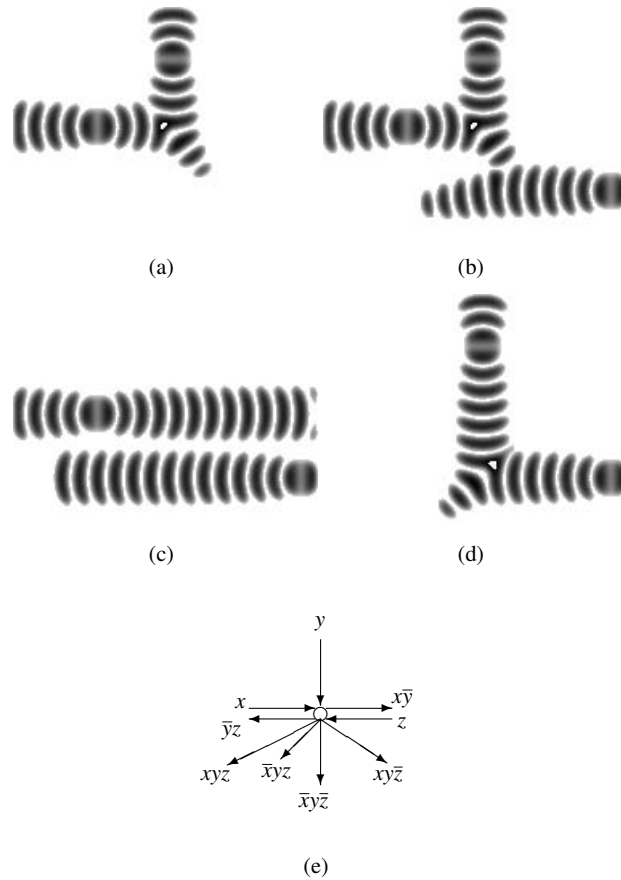
Fig. 14 Implementation of \langle x, y, z \rangle \rightarrow \langle x\bar{y}, \bar{y}z, xyz, \bar{x}yz, \bar{x}y\bar{z}, xy\bar{z} \rangle interaction gate. Overlay of images of wave fragments taken every 0.5 time units. The following combinations of input configuration are shown: (a) x = 1, y = 1, z = 0 , north-south wave collides to east-west wave. (b) x = 1, y = 1, z = 1 , north-south wave collides to east-west wave, and to west-east wave. (c) x = 1, y = 0, z = 1 , west-east and east-west wave fragments pass near each other without interaction. (d) x = 0, y = 1, z = 1 , north-south wave collides to east-west wave. (e) Scheme of the gate. From [2].
