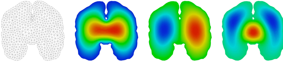
Figure 2. Initial mesh (left), initial basis functions n^{\circ}1 , n^{\circ}2 and n^{\circ}5 (right).
