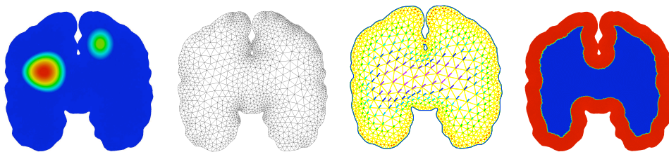
Figure 1. Unknown coefficient \bar{p} (on the left), computational mesh and initial data \bar{u}_0 (in the center), observation zone \omega (in red, on the right).
