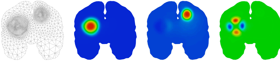
Figure 3. Adapted mesh (left), adapted basis functions n^{\circ}1 , n^{\circ}2 and n^{\circ}5 (right).
