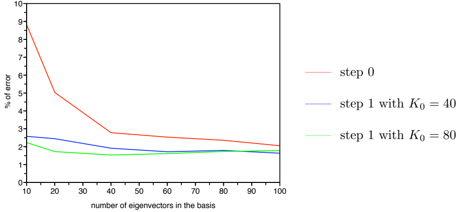
Figure 4. Relative error for the coefficient p in L^2 -norm with respect to K .
