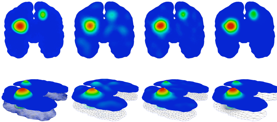
Figure 5. Exact coefficient \bar{p} (on the left), recovered coefficient p^* at step 0 with K_0 = 50 and K_0 = 100 (in the center), recovered coefficient p^* at step 2 with K_0 = K_1 = K_2 = 50 (on the right).
