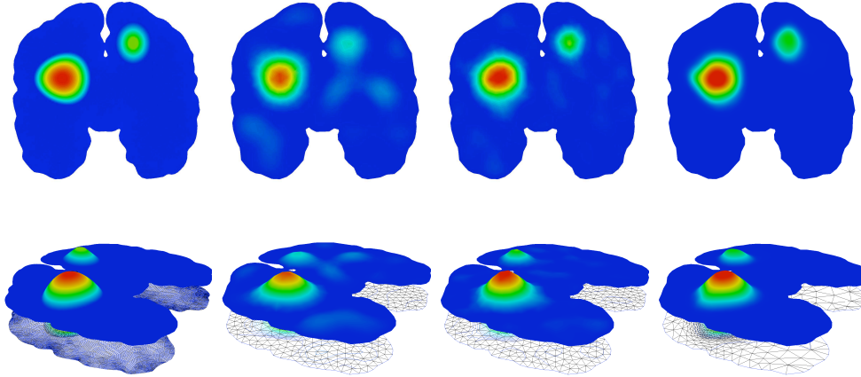
Figure 5. Exact coefficient \bar{p} (on the left), recovered coefficient p^* at step 0 with K_0 = 50 and K_0 = 100 (in the center), recovered coefficient p^* at step 2 with K_0 = K_1 = K_2 = 50 (on the right).
