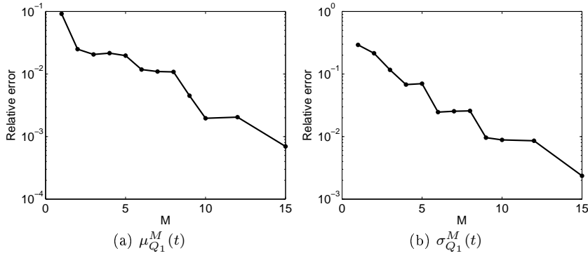
Fig. 9 Example 1. Convergence with M of the mean \mu_{Q_1}^M(t) (a) and standard deviation \sigma_{Q_1}^M(t) (b) of the quantity of interest Q_1(u_M)(t, \xi) . Relative error (in L^2(I) -norm) with respect to the reference Monte-Carlo simulations.
