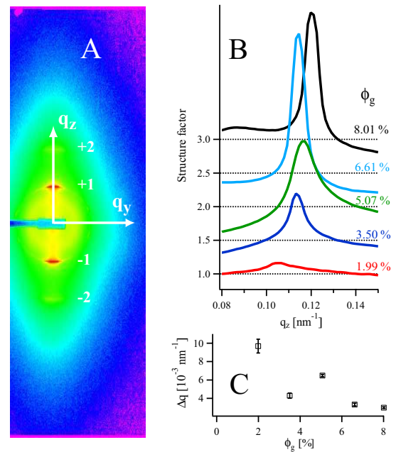
Figure 4: A – SAXS image (taken without magnetic field) of a lamellar phase containing \phi_g = 6.61 vol % goethite, aligned in planar anchoring (the layer normal is along z. ). Several Bragg peaks are visible, labelled by their index. B – Structure factors of the lamellar phase doped with increasing amounts of goethite, indicated alongside the curves. The curves are shifted vertically in steps of 0.5. C – Width of the Bragg peaks in B as a function of the goethite concentration.
