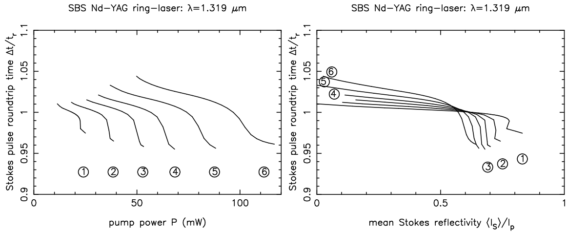
Figure 19: Numerical simulation of Eqs.(1): Stokes pulse roundtrip time at z = 0 normalized to the linear flight time \delta_t |A_S(0, t)|^2 / t_r vs . input pump power in mW (left) and vs . normalized mean Stokes reflectivity \langle |A_S(0, t)|^2 \rangle / |A_p(0)|^2 (right).
