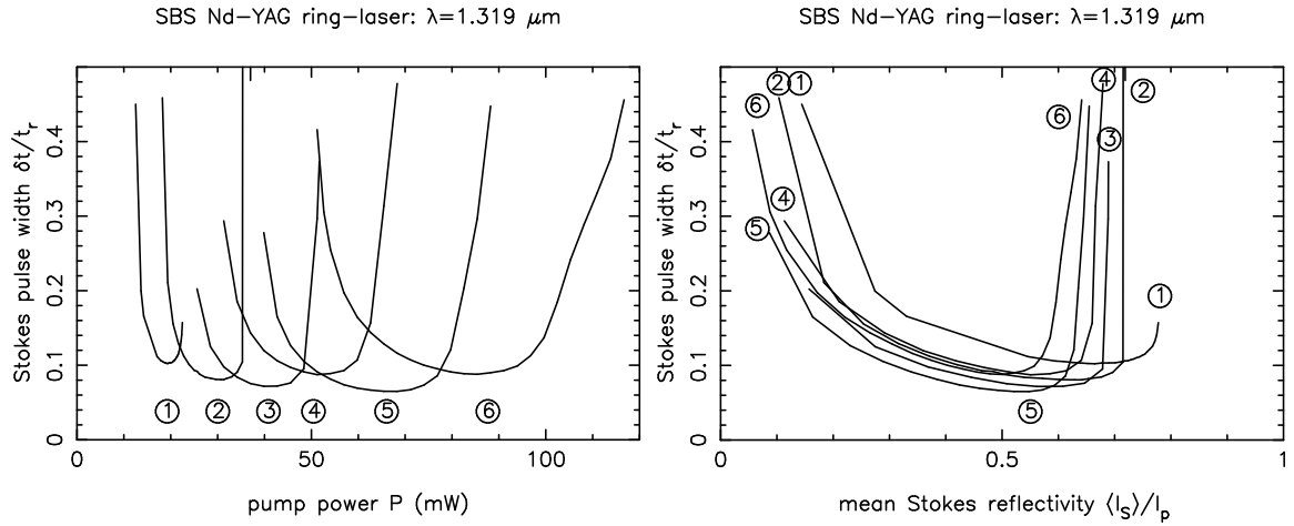
Figure 17: Numerical simulation of Eqs.(1): Stokes intensity pulse width at z = 0 normalized to the linear flight time \delta_t |A_S(0, t)|^2 / t_r vs. input pump power in mW (left) and vs. normalized mean Stokes reflectivity \langle |A_S(0, t)|^2 \rangle / |A_p(0)|^2 (right).
