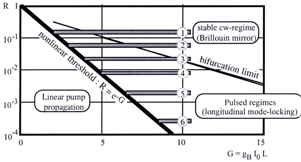
Figure 2: Bifurcation diagram of the Brillouin fiber ring laser with the experimentally explored areas (tinted areas).
