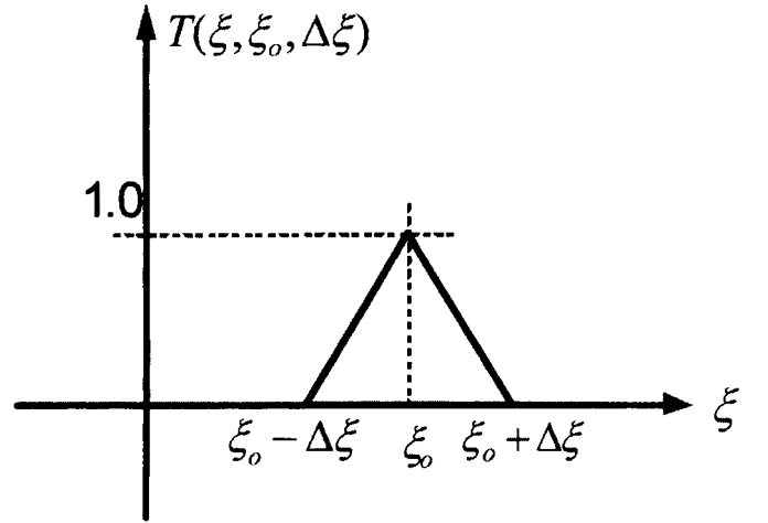
Figure 2. An illustration of the triangle function, T , defined by Equation (26).
