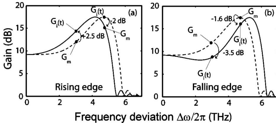
Figure 5. Parametric gain bands for (a) a rising and (b) a falling edge of the pump phase (solid lines), and for \partial\varphi/\partial\tau = 0 (dashed lines).
