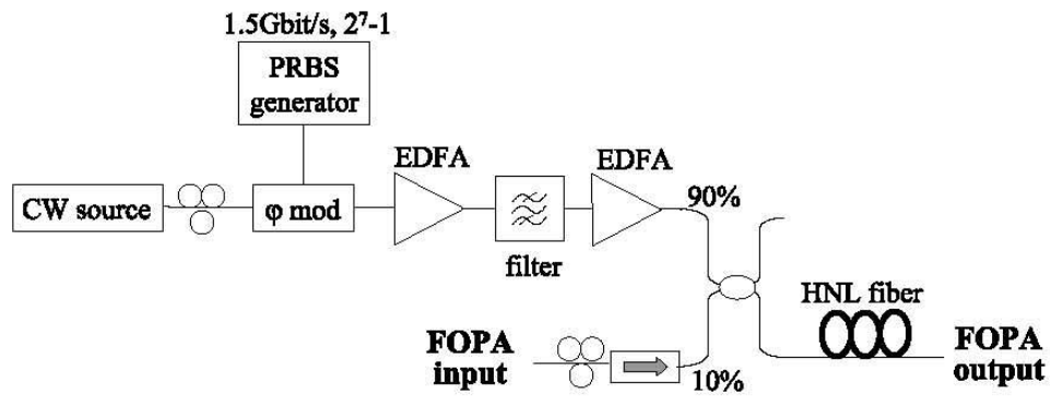
Figure 6. Experimental set-up of our fiber optical parametric amplifier under test.
