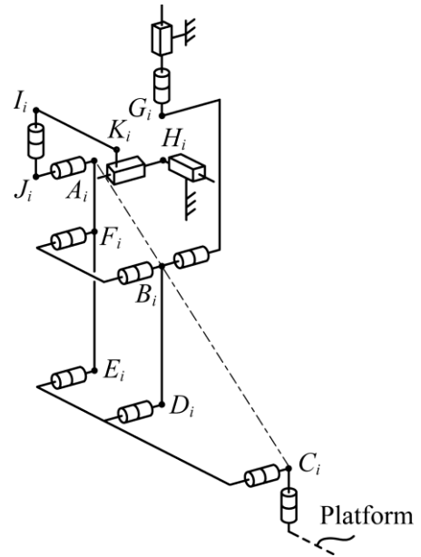
(d) the RP chain is replaced by a PRR chain.
