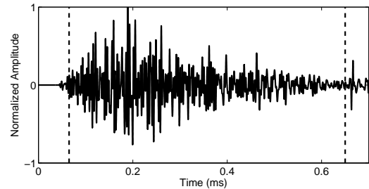
FIG. 2. Typical record collected through a concrete sample. The integration time-window is marked by the two dashed vertical lines: at 0.05 ms and at 0.65 ms. The initial impulse duration is about 10\mu s .
