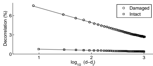
FIG. 7. Slow dynamics observed in undamaged and damaged concrete.
