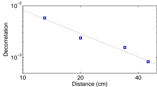
FIG. 6. Decorrelation of ultrasonic waveforms obtained a few ms right after the impact in log-log scale, at different distances from the impact. Squares are experimental data, dots represents a power law with the exponent -1.5.
