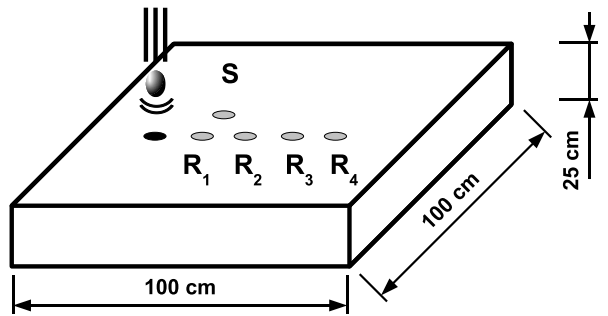
FIG. 5. Experimental setup for sample #2. Four receivers ( R_{1..4} ) are aligned with the impact location. The source S is 10 cm off the impact-receivers axis.
