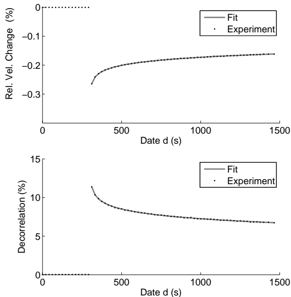
FIG. 3. Relative velocity change \delta V/V (top) and decorrelation (bottom) versus the date d of the measurement. Impact is at d_I = 270 s. Thermal effects are negligible. A logarithmic fit is added to each experimental curve.
