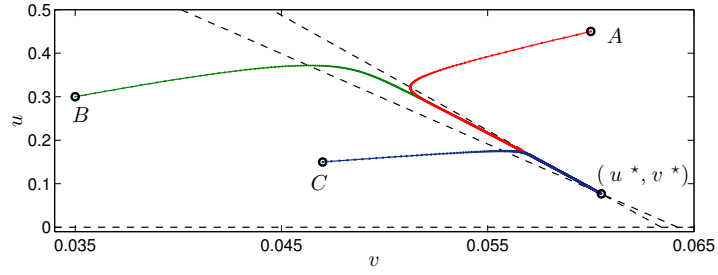
FIGURE 10. Phase portrait for the ODE system (9.2). The system nullclines (in dashed lines) are the lines u = 0 , v = 0 (not shown), v = a_1/c_1 - b_1/c_1u , v = a_2/c_2 - b_2/c_2u . Three computed trajectories are displayed starting from the states A = (0.45, 0.06) , B = (0.3, 0.035) and C = (0.15, 0.047) . After 500 time steps all of them reach the equilibrium point (u^*, v^*) = (0.0769, 0.0605) . The used parameters are a_1 = 0.61/\text{year} , a_2 = 0.52/\text{year} , b_1 = 0.4575 , b_2 = 0.31 , c_1 = 9.5 , c_2 = 8.2 .
