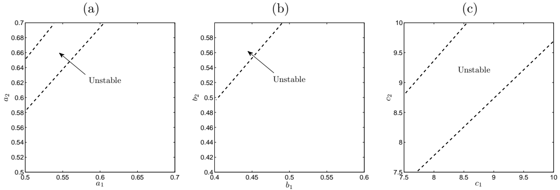
FIGURE 11. Sketched instability regions for the SKT model. The parameter spaces are determinate by fixing the remaining parameters and varying only one parameter pair: a_1, a_2 (a) b_1, b_2 (b) and c_1, c_2 (c) (Example 3).
